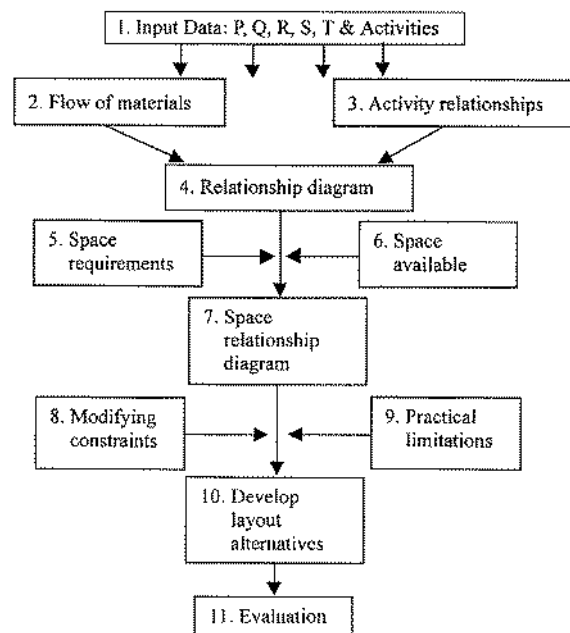
Figure 1. Diagram SLP
