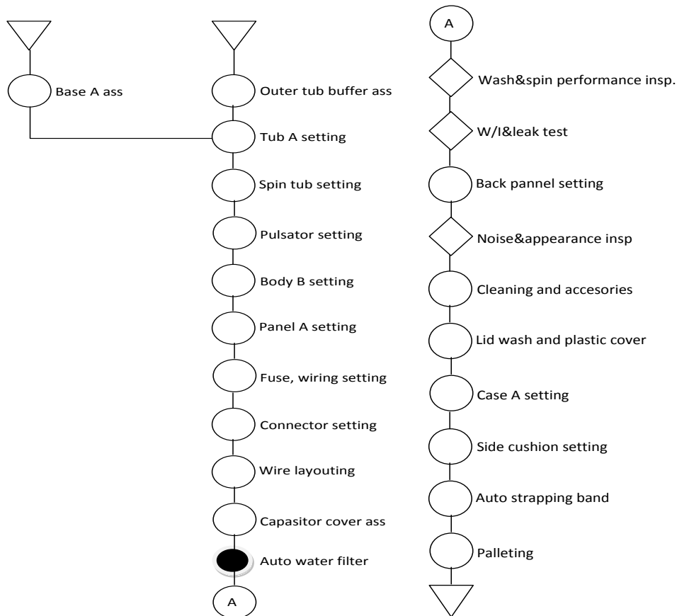
Figure 1. Process chart of washing machine assembly
